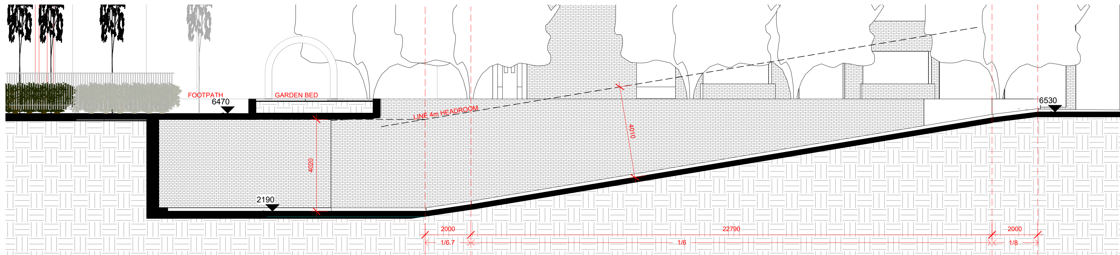
PURCHASE ST - BASEMENT RAMP SECTION
